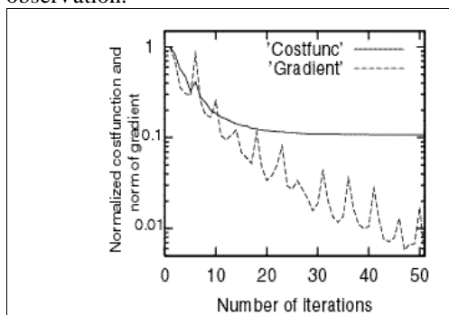
Fig 1: The scaled cost function ( J/J_0 ) (solid line), and scaled gradient norm ( \|g\|/|g_0| ) (dashed line) as a function of the number of iterations.
