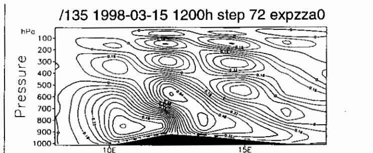
Figure 13. Cross-section of vertical velocity from integration with iterated trajectory calculation.
