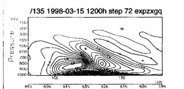
Figure 17. Cross-section of vertical velocity from experiment with all nonlinear terms decentered.
