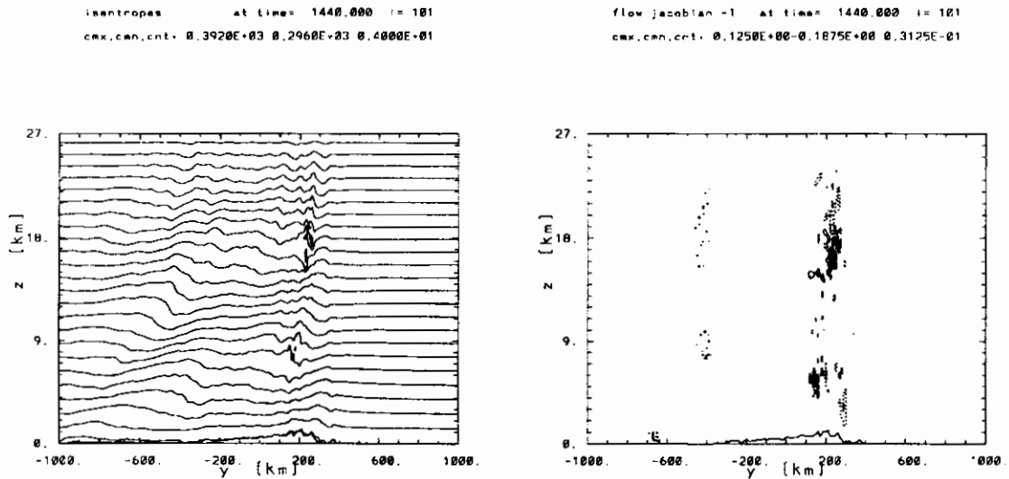
Figure 4. Cross-section of potential temperature and flow Jacobian.
