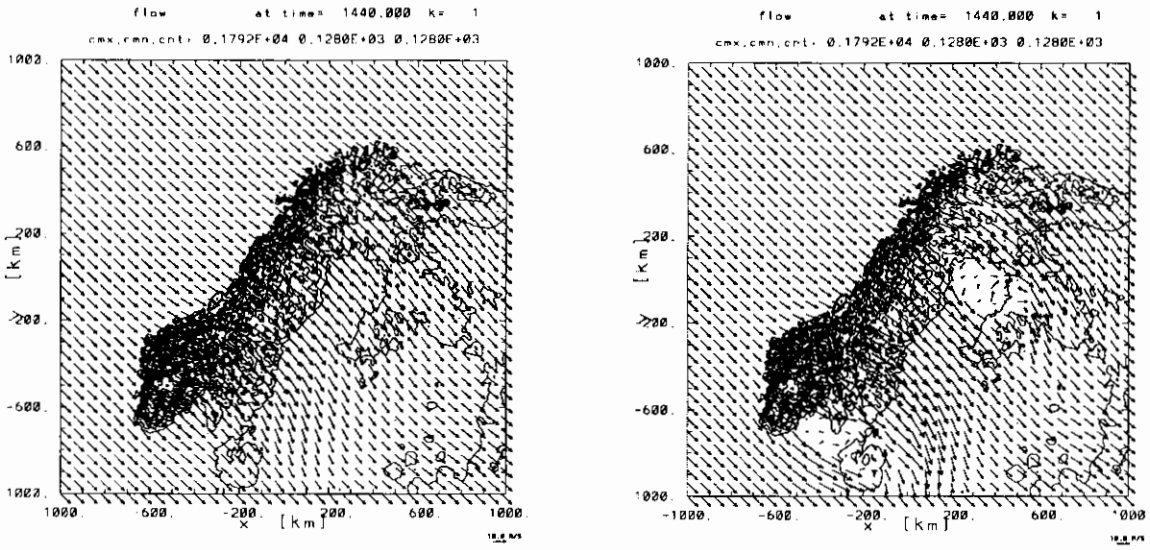
Figure 1. Comparison of solutions using explicit Eulerian (left) and semi-Lagrangian (right) schemes.
