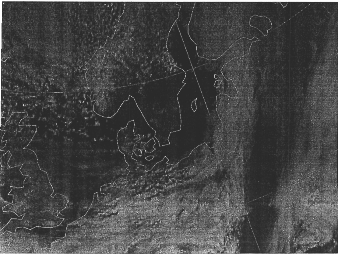
Figure 10. METEOSAT visible picture for 18 March 1998, 1200UTC.
