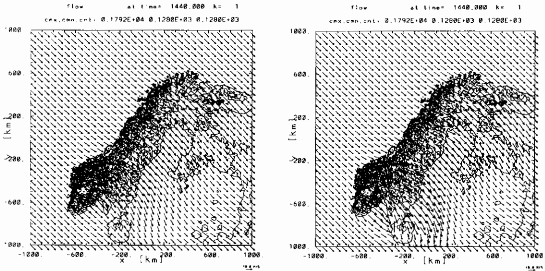
Figure 2. Comparison of semi-implicit Eulerian (left) and semi-Lagrangian (right) schemes.
