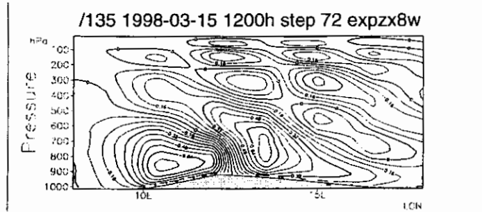
Figure 11. Cross-section of vertical velocity from control run.
