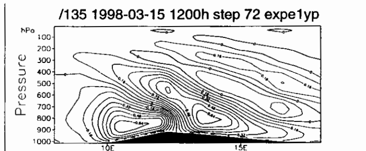
Figure 16. Cross-section of vertical velocity from experiment with decentered vertical velocity.
