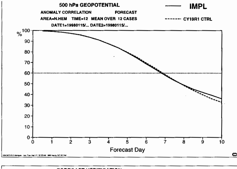
Figure 5. 500hpa scores from forecasts using iterated solver for nonlinear terms.
