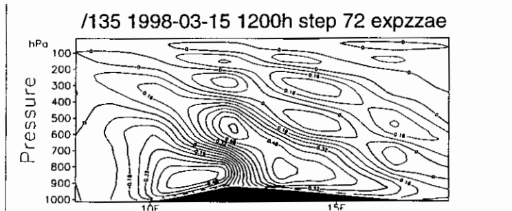
Figure 12. Cross-section of vertical velocity from integration with 5 minute timestep.
