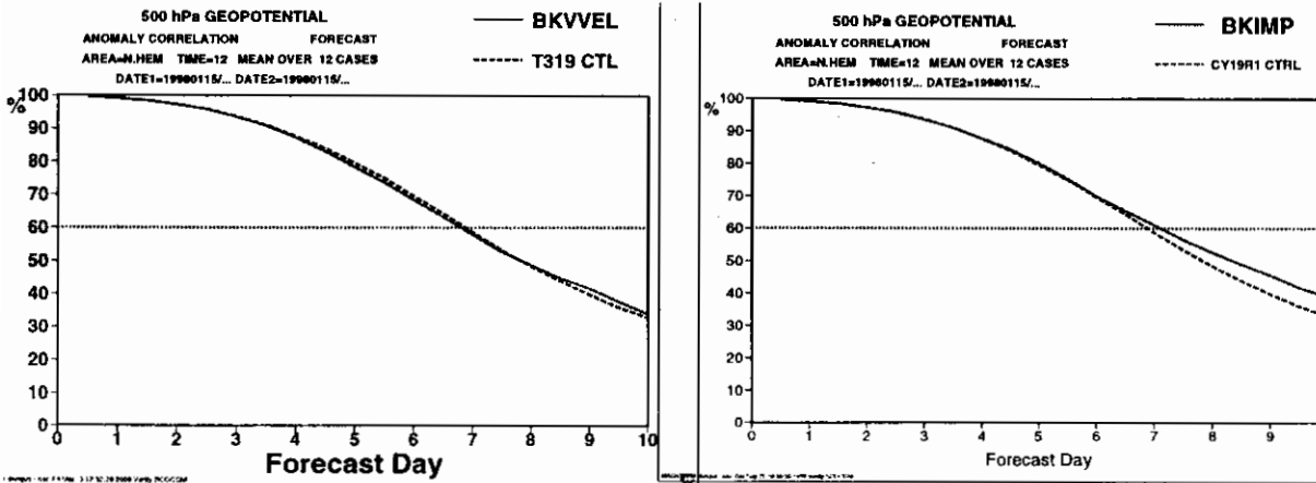
Figure 18. Performance at 500hpa of forecasts using decentring along trajectories
