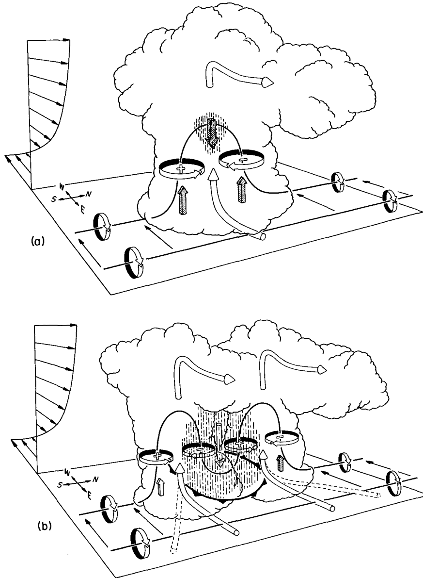
FIG. 15. Schematic depicting how a typical vortex tube contained within (westerly) environmental shear is deformed as it interacts with a convective cell (viewed from the southeast). Cylindrical arrows show the direction of cloud-relative airflow, and heavy solid lines represent vortex lines with the sense of rotation indicated by circular arrows. Shaded arrows represent the forcing influences that promote new updraft and downdraft growth. Vertical dashed lines denote regions of precipitation. (a) Initial stage: vortex tube loops into the vertical as it is swept into the updraft. (b) Splitting stage: downdraft forming between the splitting updraft cell tilts vortex tubes downward, producing two vortex pairs. The barbed line at the surface marks the boundary of the cold air spreading out beneath the storm (from Klemp 1987).
