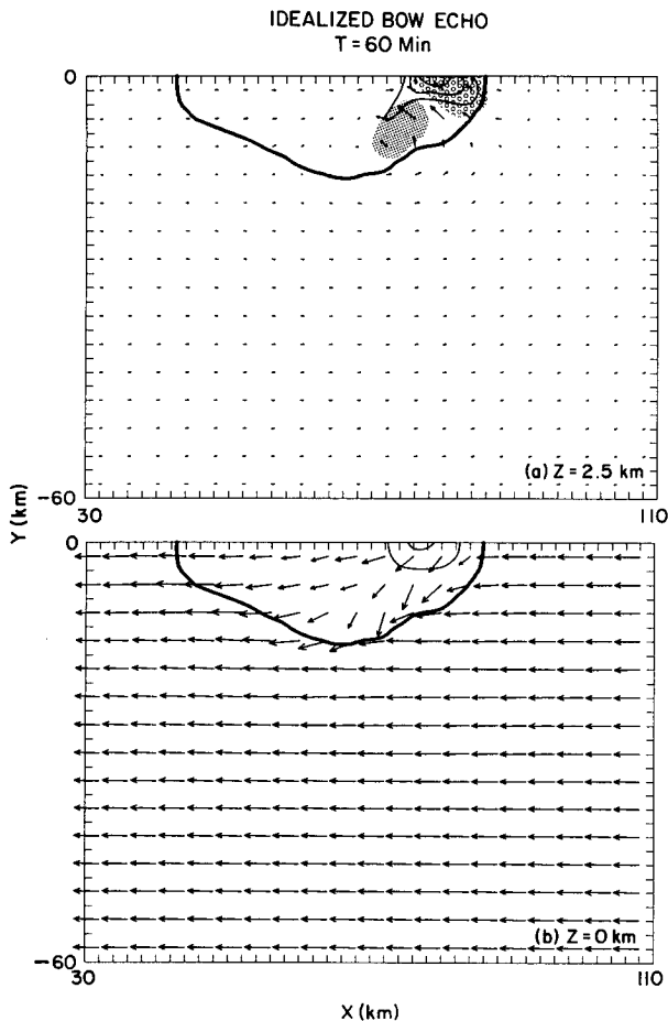
FIG. 5. Horizontal cross sections of rainwater concentration and flow vectors at (a) 2.5 km AGL and (b) 0 km AGL at 60 min for the idealized bow echo simulation. Vectors are presented at every other grid point, with a vector length of two grid intervals being equal to a magnitude of 25 \text{ m s}^{-1} . A domain speed of U = 22.5 \text{ m s}^{-1} is subtracted from the flow field. The ground-relative system propagation speed at this time is 18 \text{ m s}^{-1} . The rainwater is contoured at 2 \text{ g kg}^{-1} intervals, and the thick line represents the location of the gust front at the surface. For (a), regions of updraft greater than 4 \text{ m s}^{-1} are shaded and regions of downdraft less than -2 \text{ m s}^{-1} are stippled. The y = 0 boundary represents the axis of symmetry for the simulation, with only a 60 \text{ km} \times 80 \text{ km} portion of the full domain presented.
