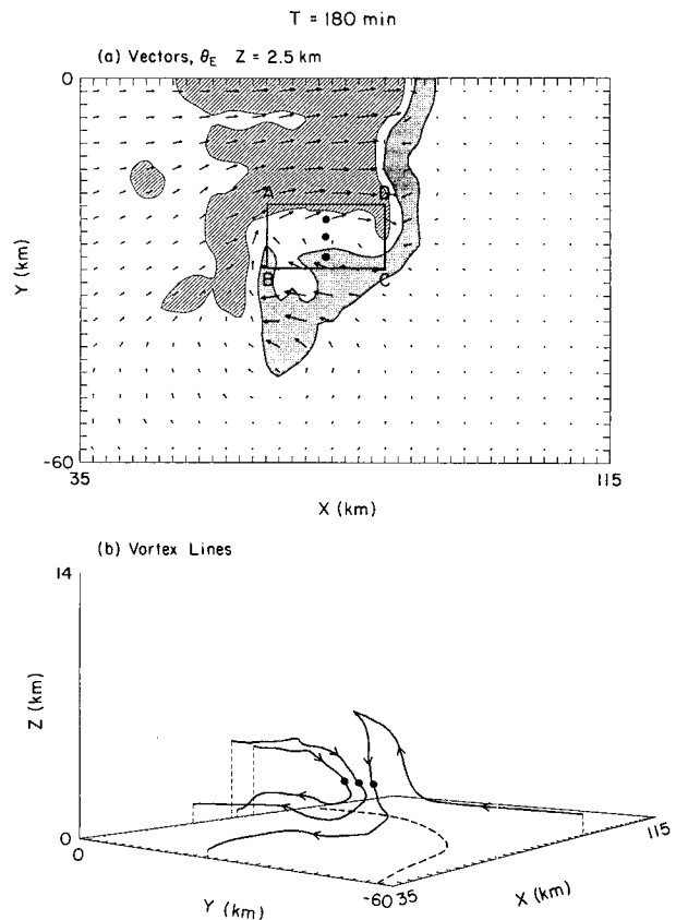
FIG. 17. Same as Fig. 16 but at t = 180 min. The ground-relative system propagation speed at this time is 27 \text{ m s}^{-1} . The box in (a) denotes the location of a circuit that is followed over time in Fig. 19.
