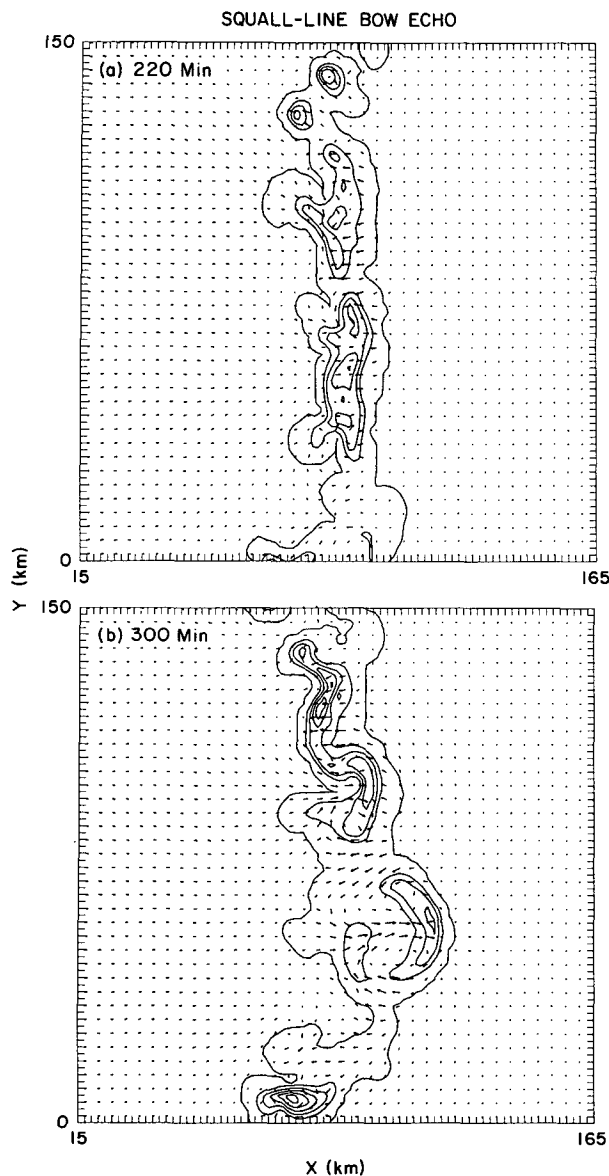
FIG. 2. Horizontal cross sections of system-relative flow and rainwater contours at 2.5 km AGL at (a) 220 min and (b) 300 min for the squall line simulation described by WKR, using an environmental vertical wind shear of 25 \text{ m s}^{-1} over the lowest 2.5 km AGL. A domain speed of U = 22.5 \text{ m s}^{-1} has been subtracted from the flow vectors. Vectors are plotted at every other grid point (a distance of two grid lengths represents 25 \text{ m s}^{-1} ). The rainwater field is contoured using a 2 \text{ g kg}^{-1} interval. Only a 150 \text{ km} \times 150 \text{ km} portion of the entire domain is shown.
