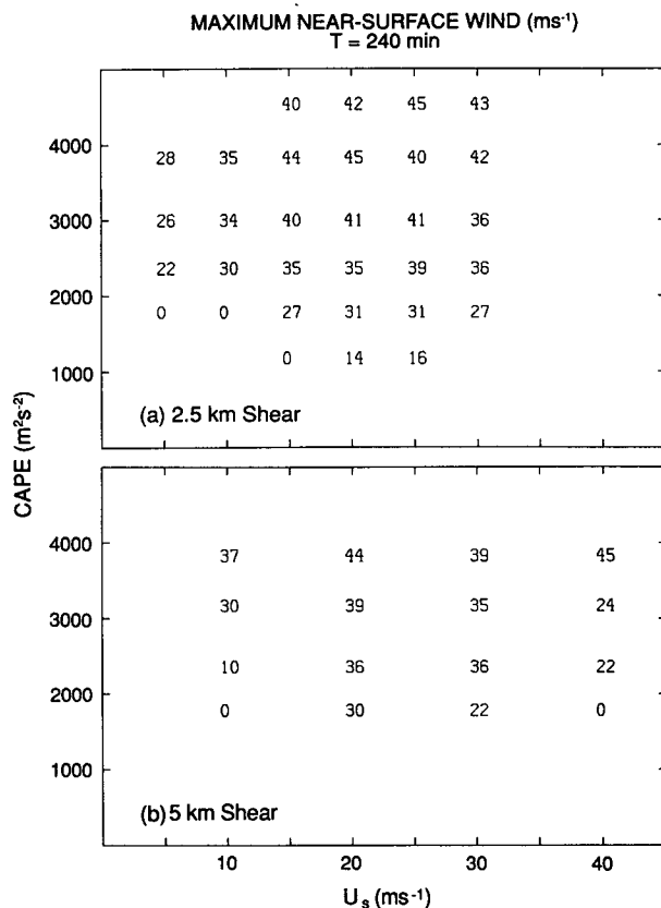
FIG. 25. Maximum near-surface (350 m AGL) wind ( \text{m s}^{-1} ) for the (a) 2.5-km shear and (b) 5-km shear experiments at t = 240 min. U_s represents the maximum magnitude of the wind for each wind profile.
