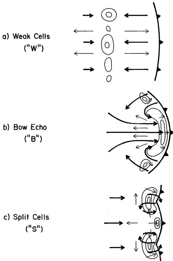
FIG. 23. Schematic depiction of the primary modes of convective organization identified in the sensitivity experiments between 180 and 240 min. Thick and thin arrows represent system-relative flow at 2.5 km AGL and the surface, respectively. Contours represent rainwater concentration. Thick barbed line represents the location of the surface gust front.
