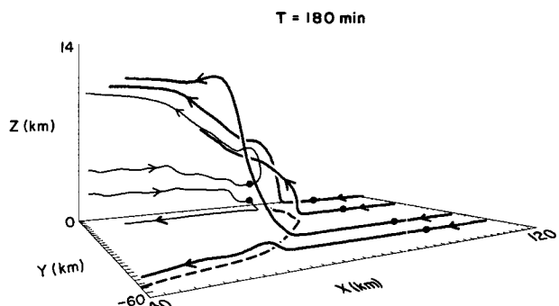
FIG. 10. Representative parcel trajectories for the idealized bow-echo simulation at 180 min. Dots represent the point of origin of each trajectory, with the trajectory integrated forward and backward in time from that point. The surface gust front at t = 180 \text{ min} is denoted by the dashed line.
