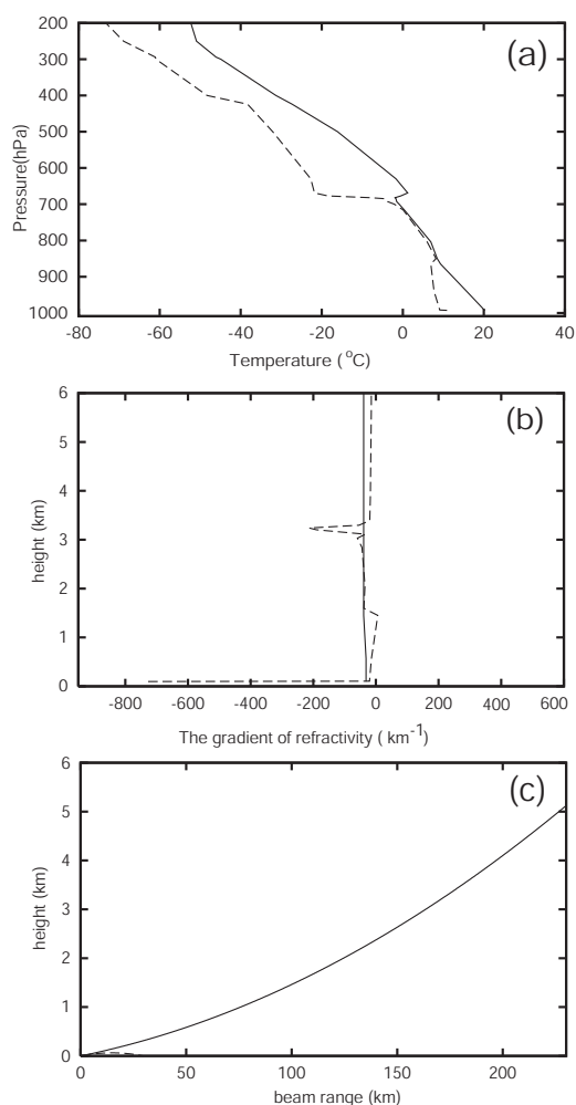
Fig. 2. (a) The temperature (solid) and dewpoint (dashed) profiles, (b) the refractivity gradient profiles ( \text{km}^{-1} ) calculated from the U.S. Standard Atmosphere (solid) and from the observed sounding (dashed), and (c) the radar ray paths calculated for the 0.5^\circ elevation using the Standard Atmosphere (solid) and actual sounding and ray tracing method (dashed, only clear in between 0–50 km), for 0000 UTC 3 May 1999 at Topeka, Kansas (TOP).
