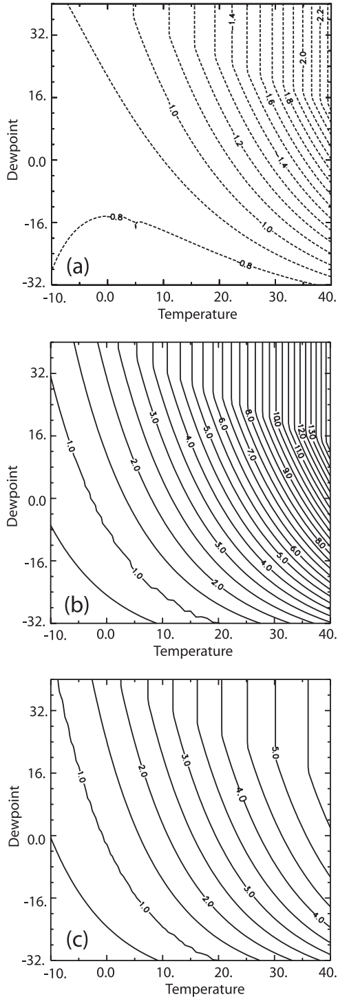
Fig. 1. The variation of refractivity with respect (a) to temperature ( ^{\circ}\text{C} ) indicated by the contours of A \equiv \partial N / \partial T in (11), and (b) to dewpoint ( ^{\circ}\text{C} ) indicated by the contours of B \equiv \partial N / \partial T_d in (12), and (c) the absolute ratio between B and A .
