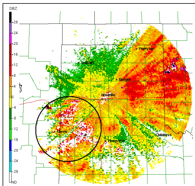
Fig. 4. Radar reflectivity (dBZ) image at 1347 UTC 8 June 2005 for KAMA at Amarillo, Texas.
